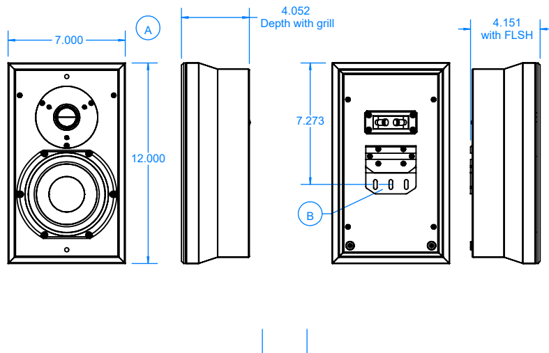
Front view shown with grill removed
