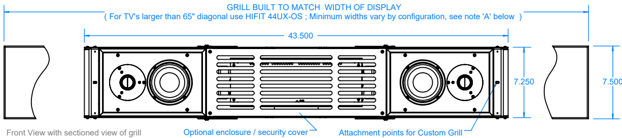
Front View with sectioned view of grill
