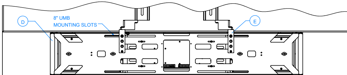
Back View with UnderMount Bracket and custom width grill
