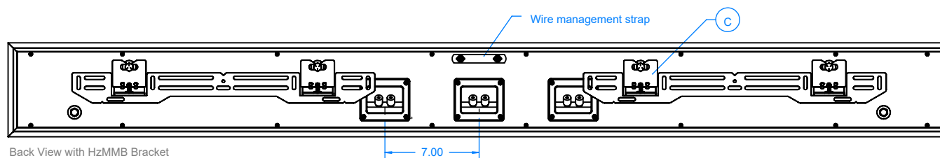
Back View with HzMMB Bracket
