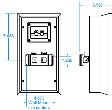
Rear and Side view with DsFMB
