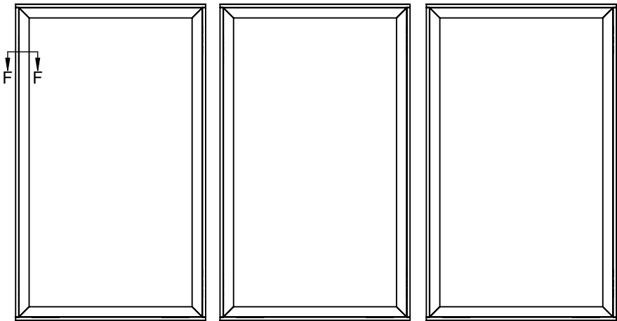
FRONT VIEW CASING & MAGNETIC TRIM ASSEMBLIES SCALE 1 : 30
