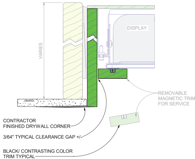
A SIMPLE CASED OPENING
