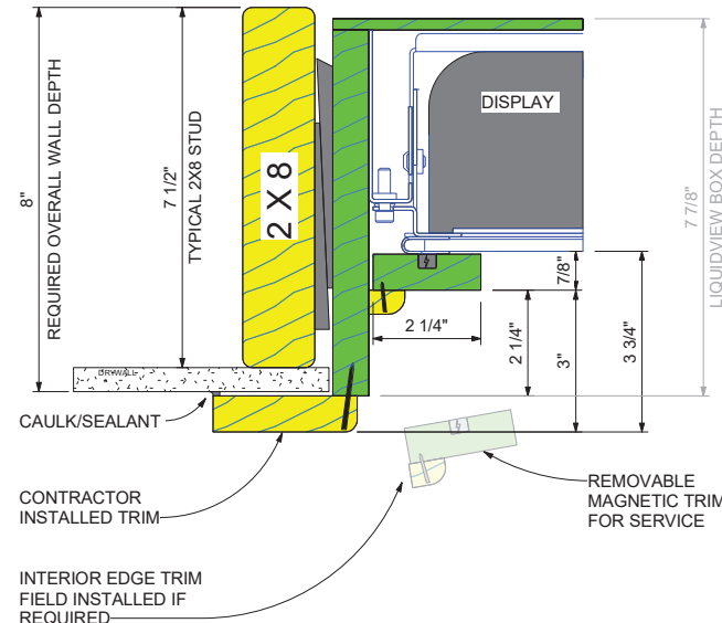
2 2 X 8 WALL (TYPICAL)
