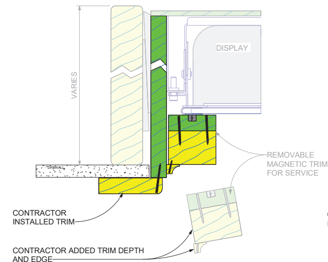
B CONTRACTOR AUGMENTED TRIM 2X8 AND 2X10 APPLICATIONS
