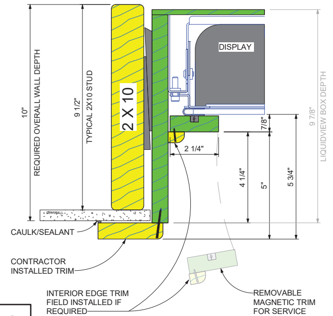
3 2 X 10 WALL (CUSTOM*)
