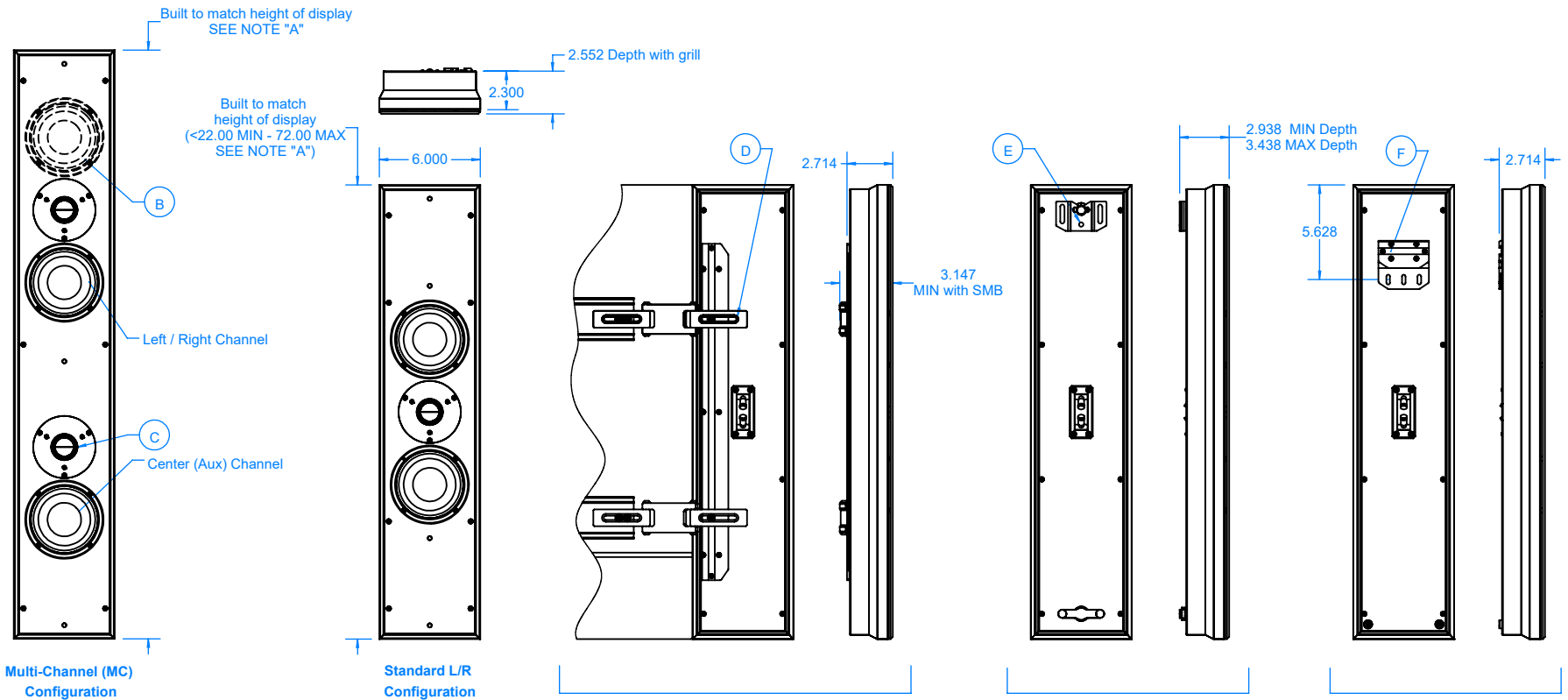
Rear and Side elevation view with PrSMB
